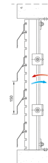
Louvre pitch 150
